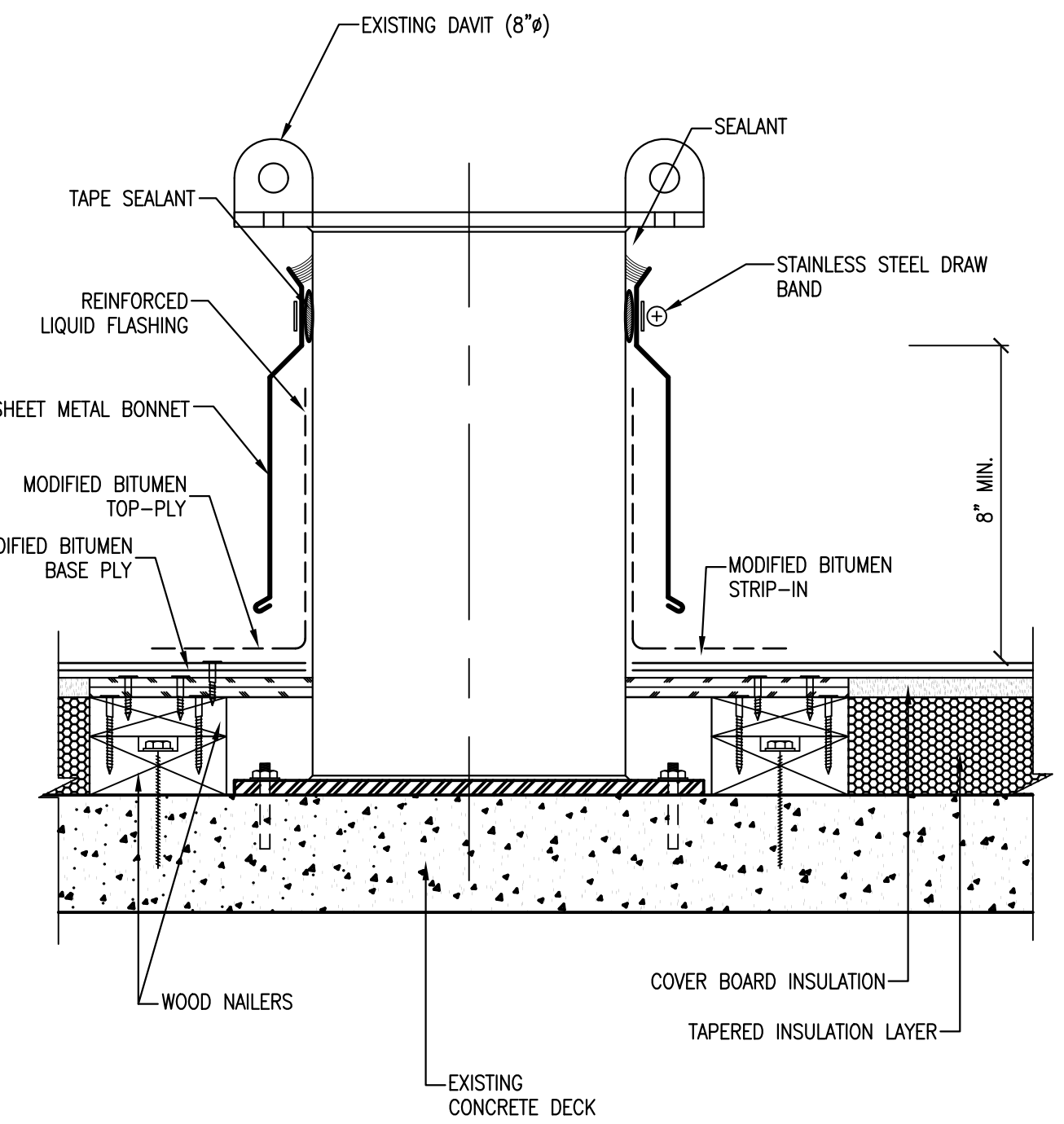
11 DAVIT R5.01 SCALE: NOT TO SCALE (TYPICAL)
