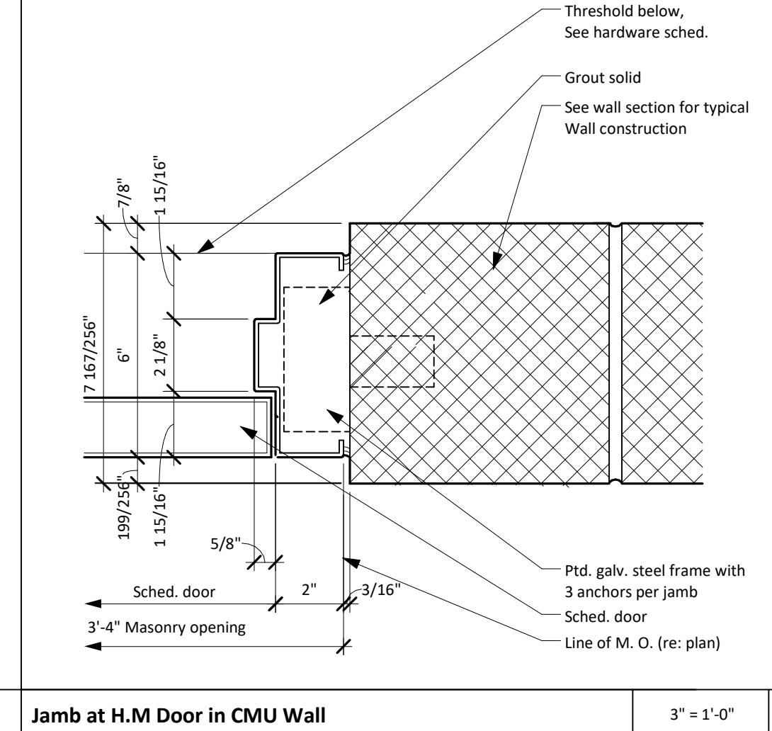
Jamb at H.M Door in CMU Wall 3" = 1'-0" 18
