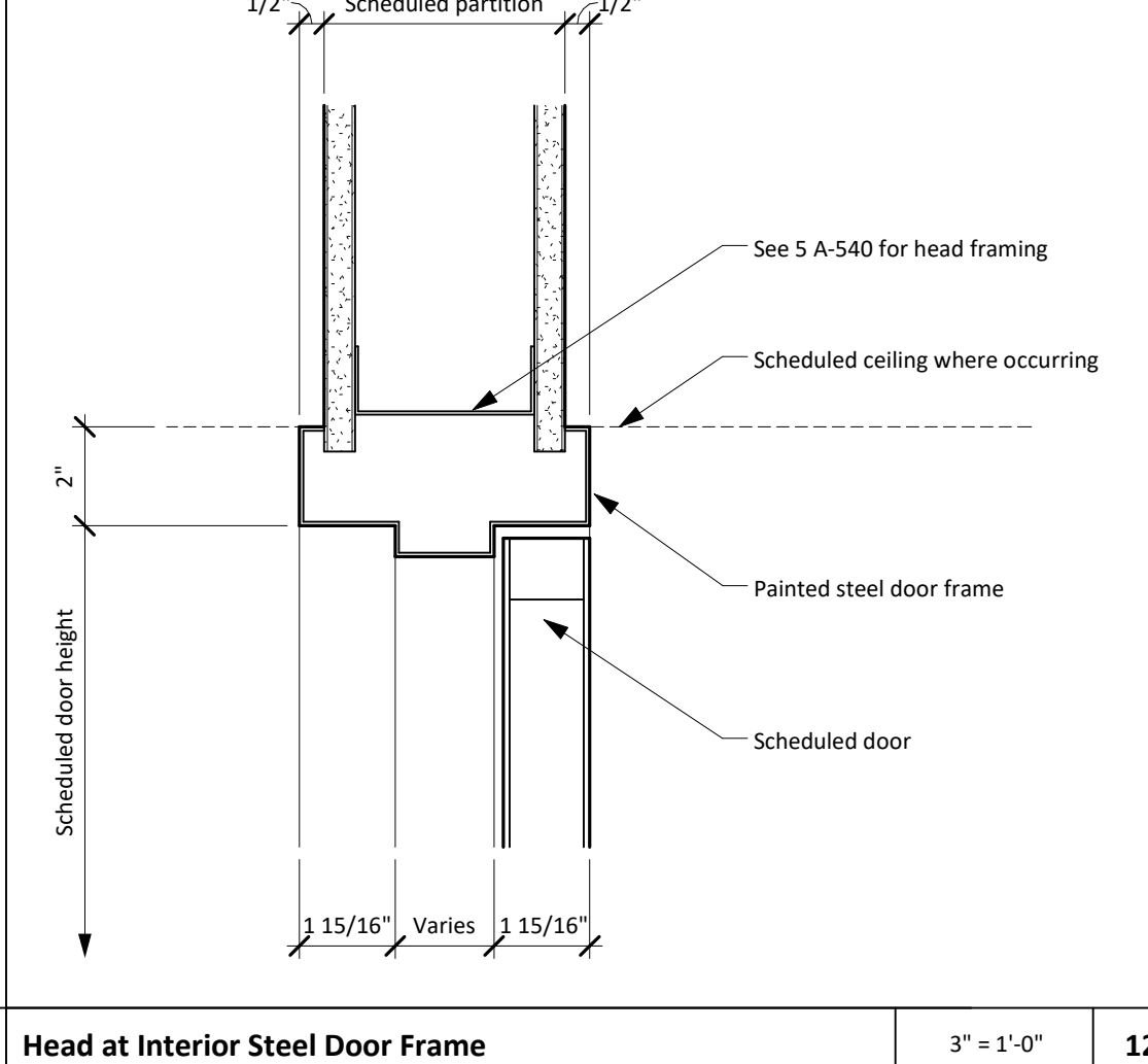
Head at Interior Steel Door Frame 3" = 1'-0" 12
