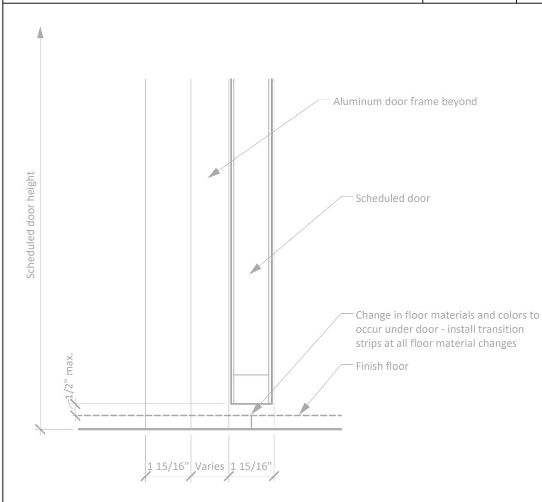
Sill at Interior Aluminum Door Frame 3" = 1'-0" 14
