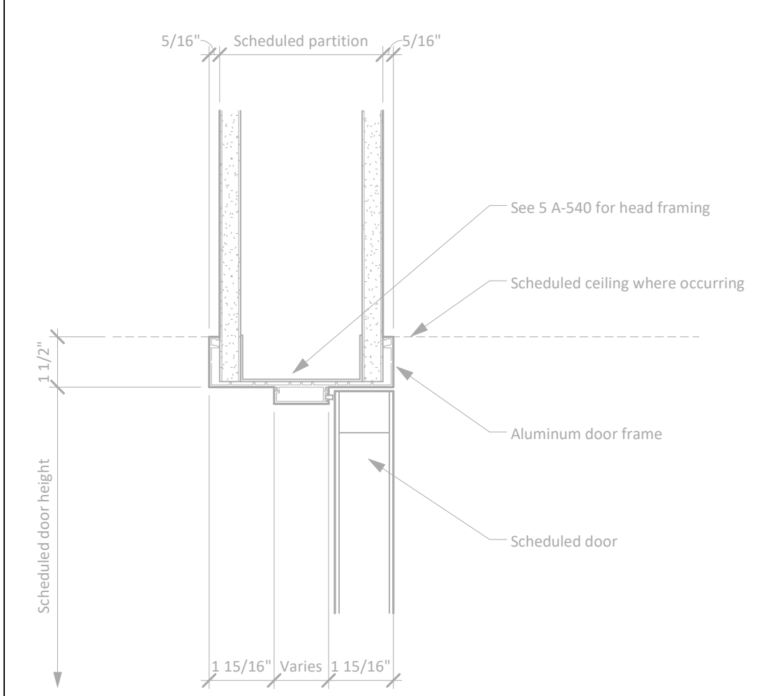
Head at Interior Aluminum Door Frame 3" = 1'-0" 15
