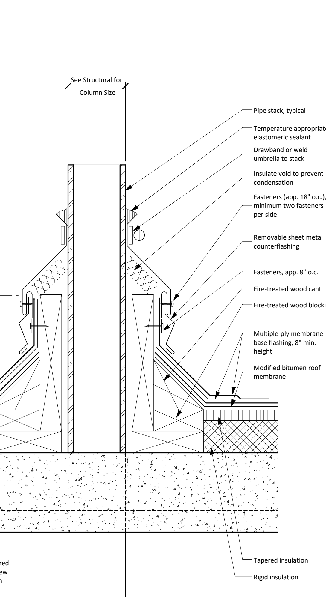
Typical Pipe Roof Penetration Detail 3" = 1'-0" 21
