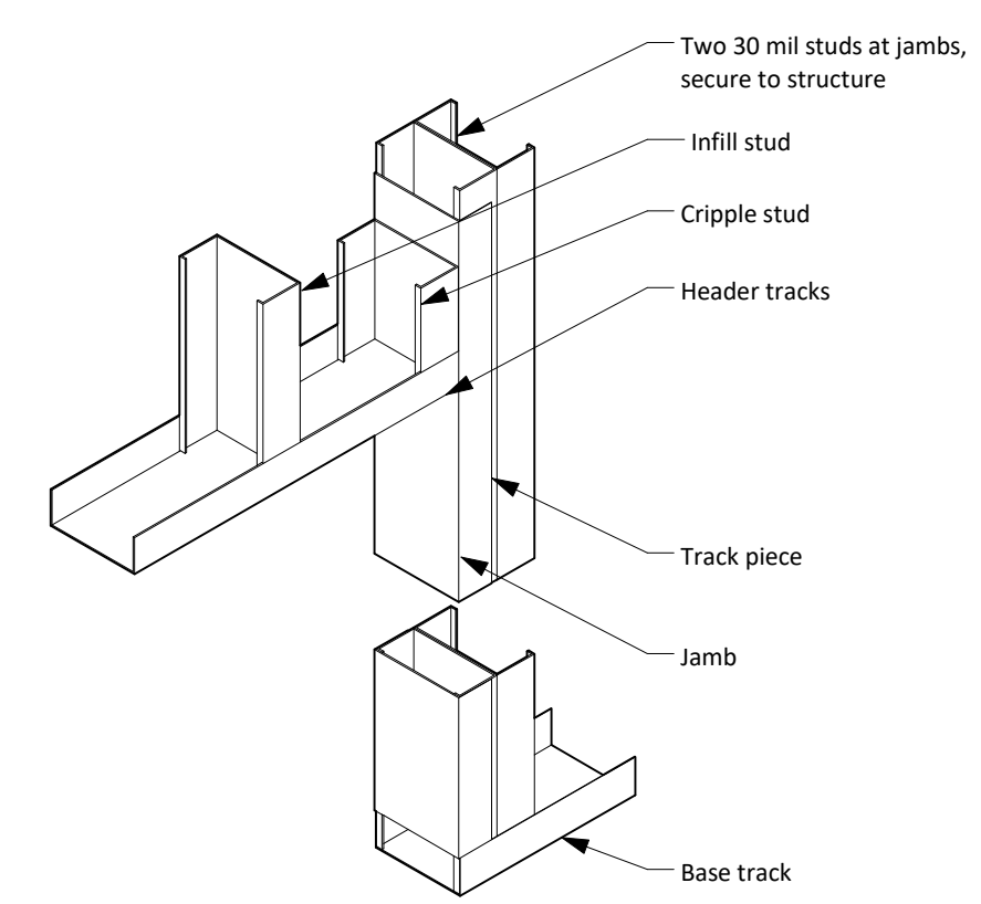
Typical Framing at Opening 3" = 1'-0" 10 N.T.S. 5
