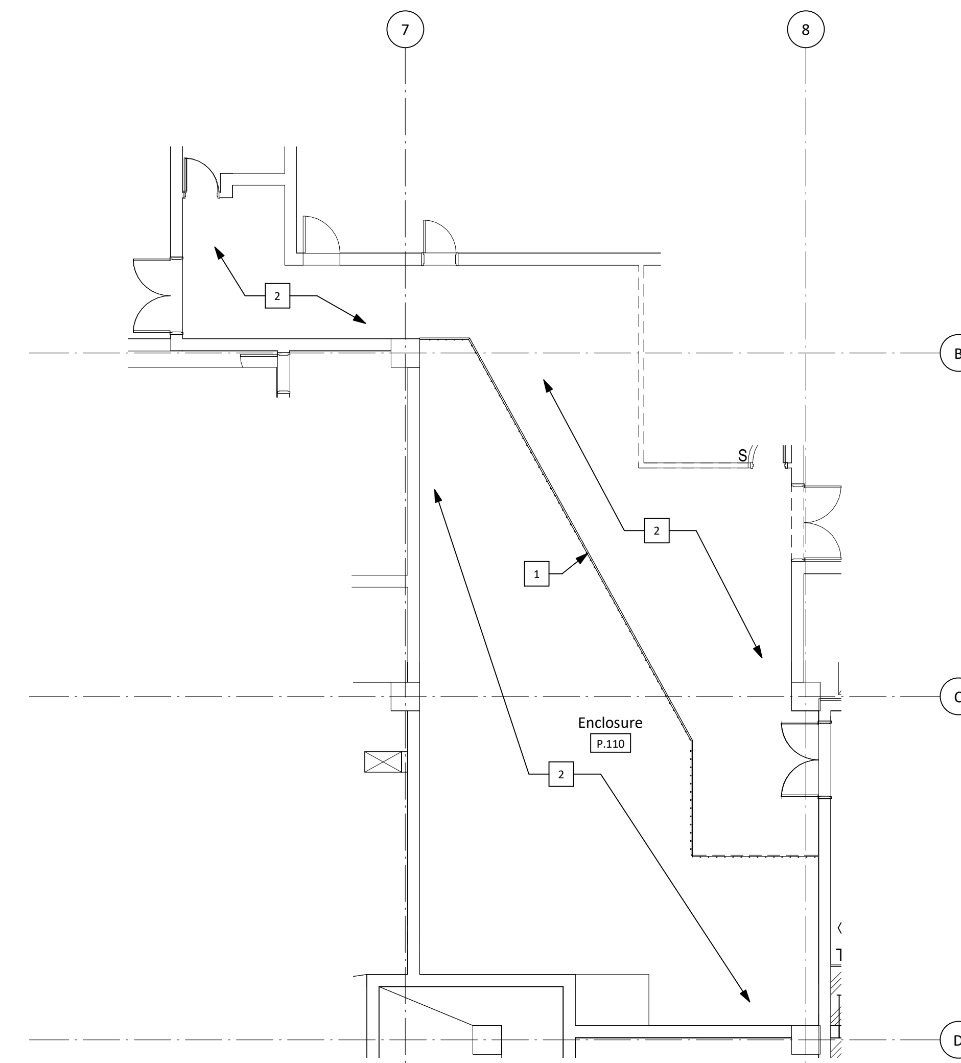
Penthouse Level Demolition RCP - Storage Plan Alternate 1/8" = 1'-0" 3
