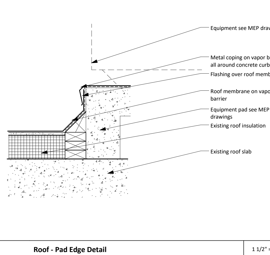
Roof - Pad Edge Detail 1 1/2" = 1'-0" 1
