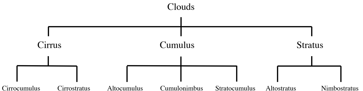
Figure 7 • Cloud Hierarchy.
