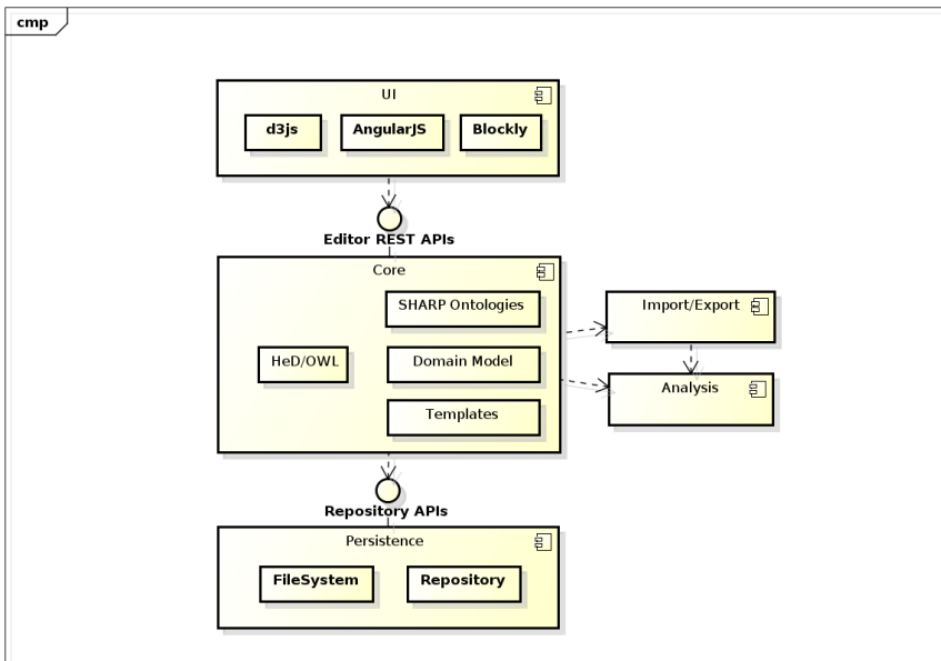
Figure 2. Implementer's Workbench conceptual architecture.
